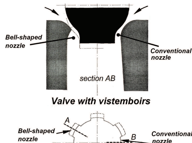
Figure 4. Control valve with vistemboirs.
