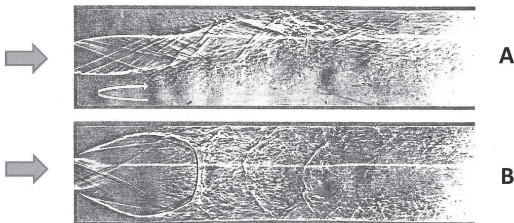
Figure 1. Schlieren visualizations obtained before (A) and after (B) spatiotemporal chaos in a two-dimensional sudden enlargement.
