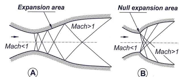
Figure 3. Conventional (A) and Bell-shaped nozzles (B).
